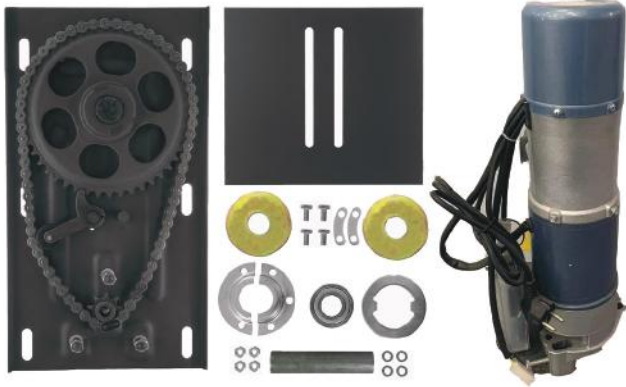
Side motor
